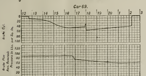
STANDING TEST OF 100-CAR A. S. A. TRAIN. VIRGINIAN RAILWAY, PRINCETON, WEST VIRGINIA, ON JULY 2nd, 1918.
